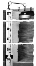
S&J 92302 Liquid Level Indicator
